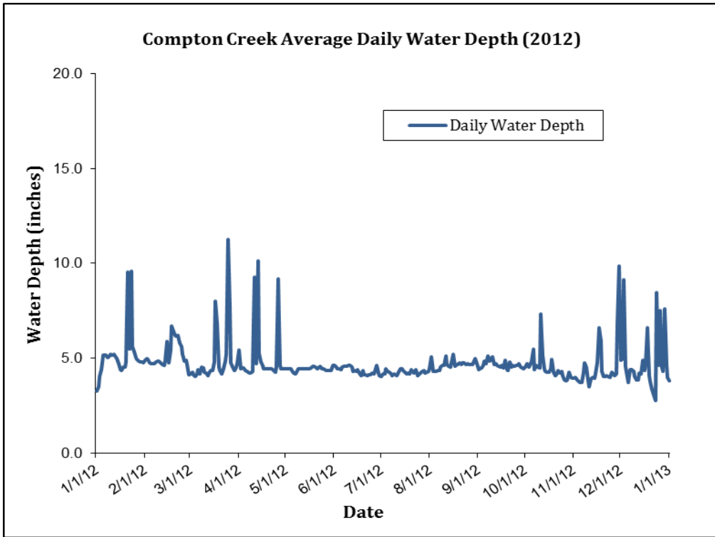
FIGURE 5-2.2a DAILY AVERAGE FLOW IN COMPTON CREEK FOR THE YEAR 2012
