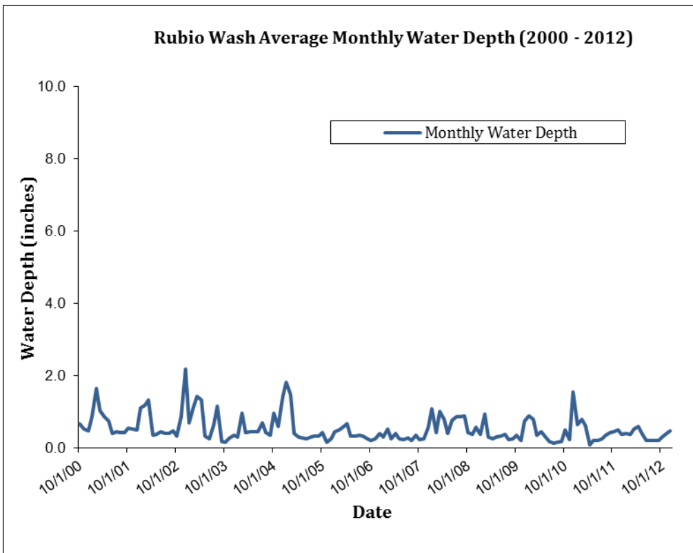
FIGURE 5-3.6: MONTHLY AVERAGE FLOW IN RUBIO WASH FROM 2000 TO 2012
