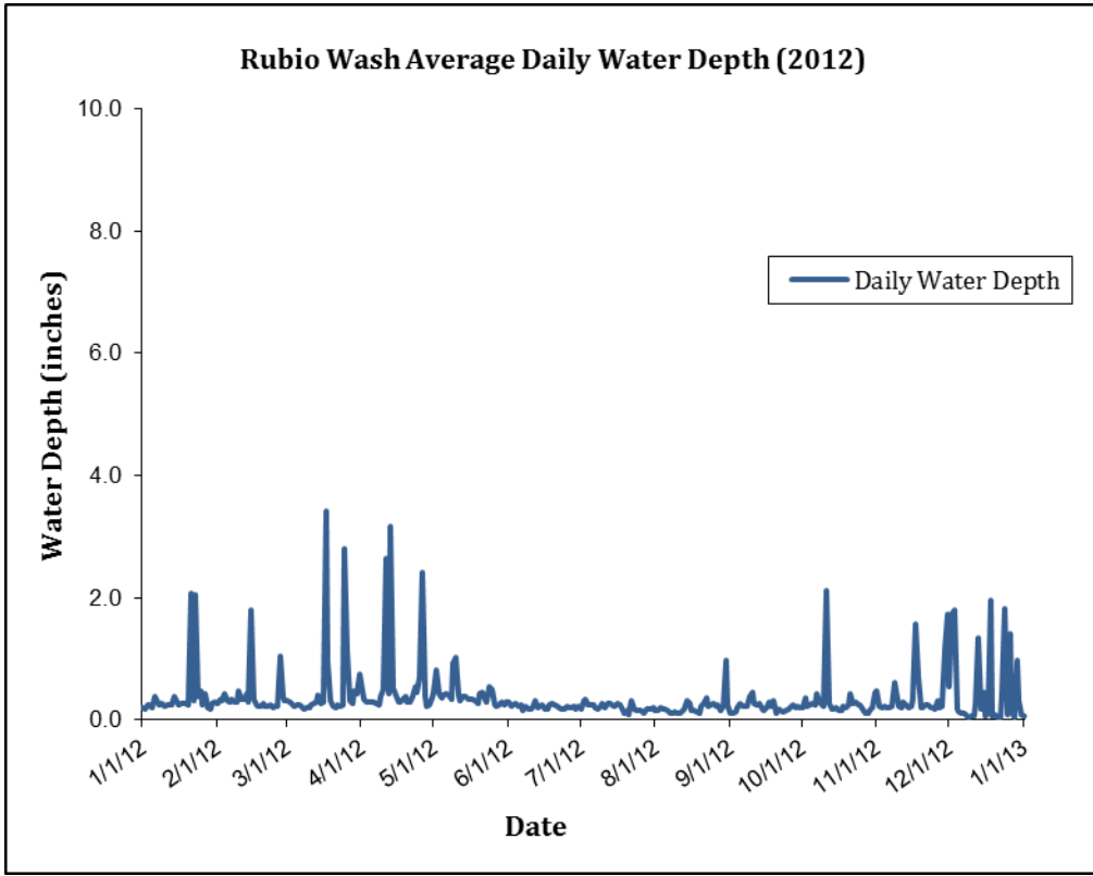
FIGURE 5-3.6a: DAILY AVERAGE FLOW IN RUBIO WASH FOR THE YEAR 2012
