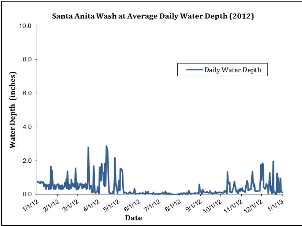
FIGURE 5-3.3a DAILY AVERAGE FLOW IN SANTA ANITA WASH FOR THE YEAR 2012
