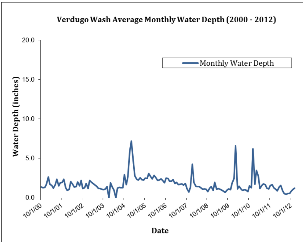
FIGURE 5-4.2b MONTHLY AVERAGE FLOW IN VERDUGO WASH FROM 2000 TO 2012
