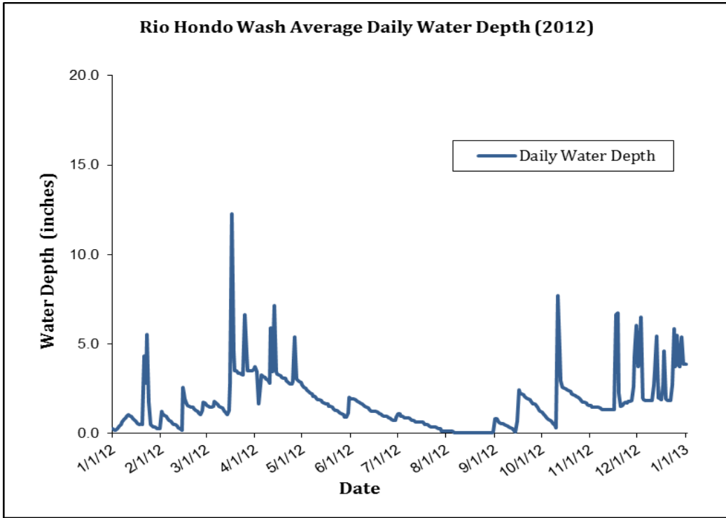
FIGURE 5-2.5a DAILY AVERAGE FLOW IN RIO HONDO FOR THE YEAR 2012
