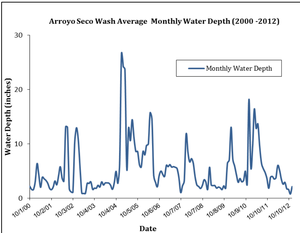
FIGURE 5-2.8b MONTHLY AVERAGE FLOW IN ARROYO SECO FROM 2000 TO 2012
