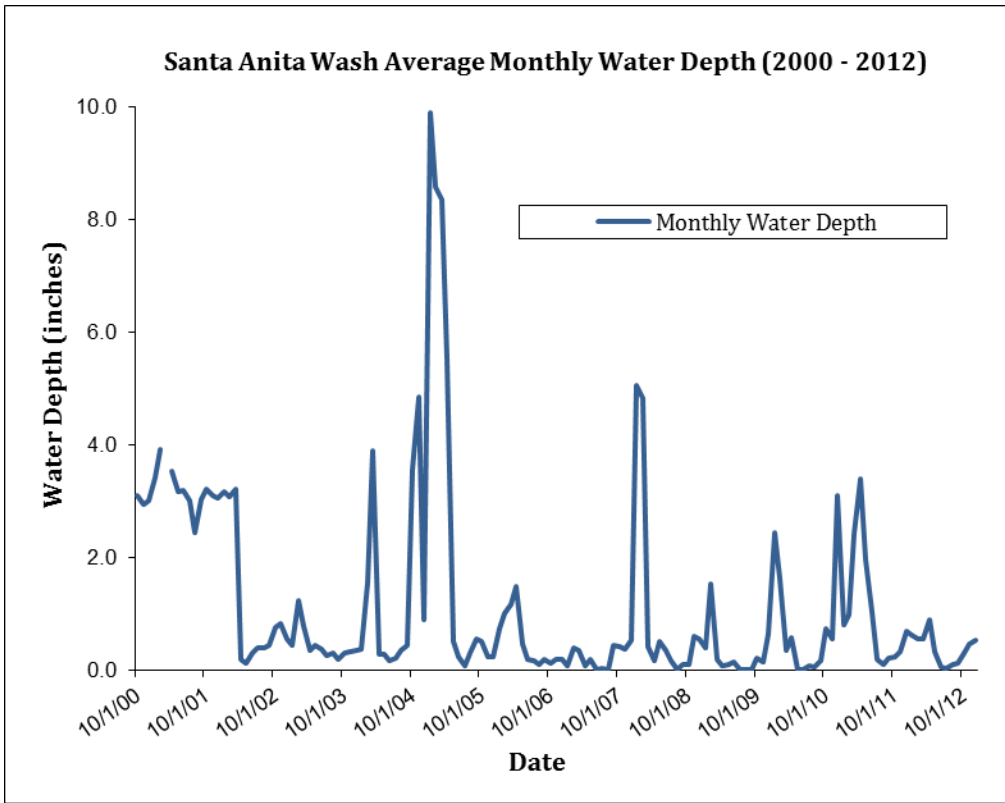
FIGURE 5-3.3b MONTHLY AVERAGE FLOW IN SANTA ANITA WASH FROM 2000 TO 2012
