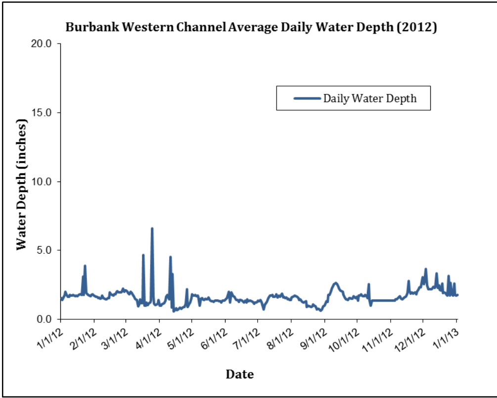
FIGURE 5-4.5a DAILY AVERAGE FLOW IN BURBANK WESTERN CHANNEL FOR THE YEAR 2012
