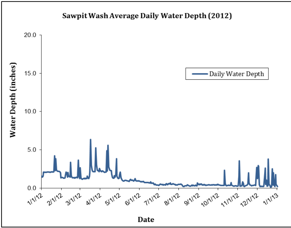
FIGURE 5-3.14a DAILY AVERAGE FLOW IN SAWPIT WASH FOR THE YEAR 2012
