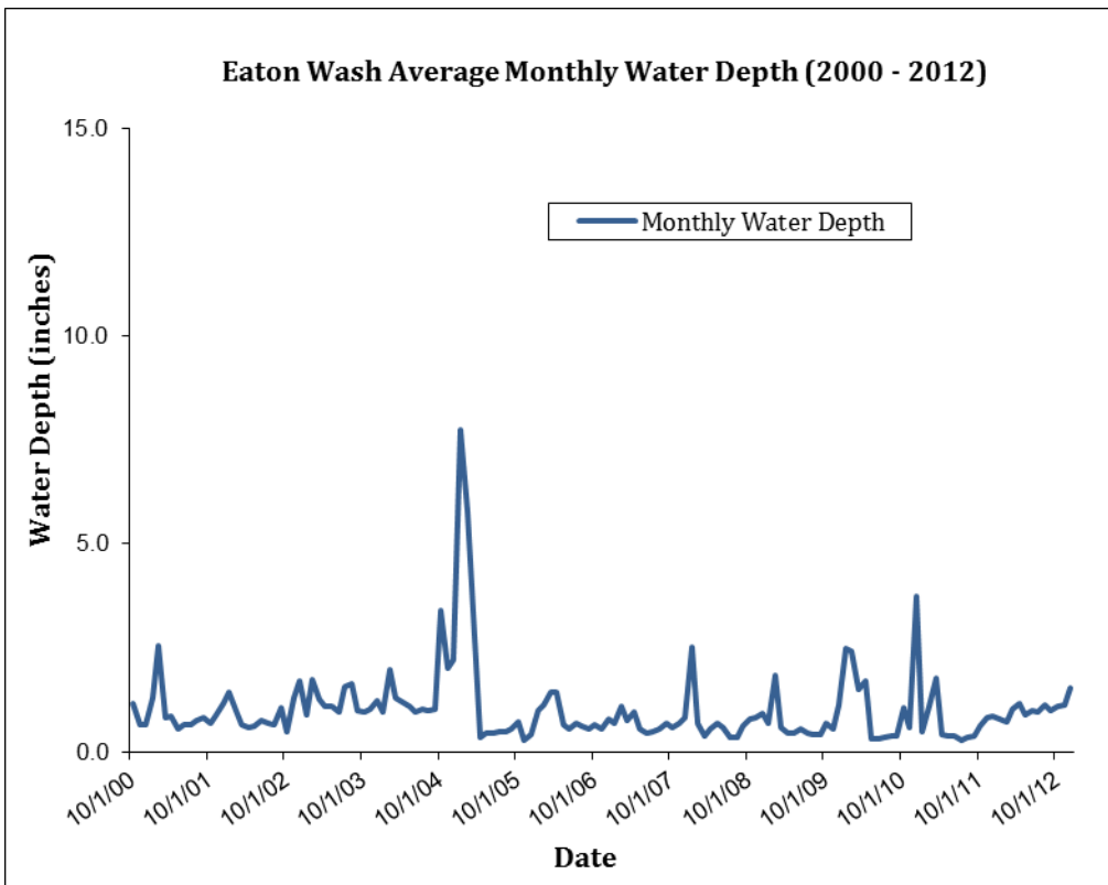
FIGURE 5-3.4b MONTHLY AVERAGE FLOW IN EATON WASH FROM 2000 TO 2012
