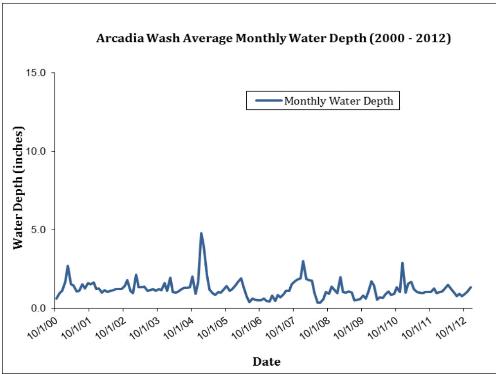
FIGURE 5-3.11b MONTHLY AVERAGE FLOW IN ARCADIA WASH FROM 2000 TO 2012
