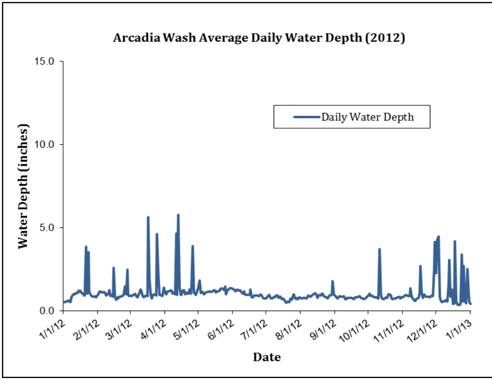
FIGURE 5-3.11a DAILY AVERAGE FLOW IN ARCADIA WASH FOR THE YEAR 2012
