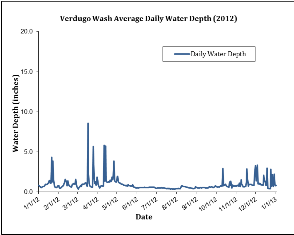
FIGURE 5-4.2a DAILY AVERAGE FLOW IN VERDUGO WASH FOR THE YEAR 2012
