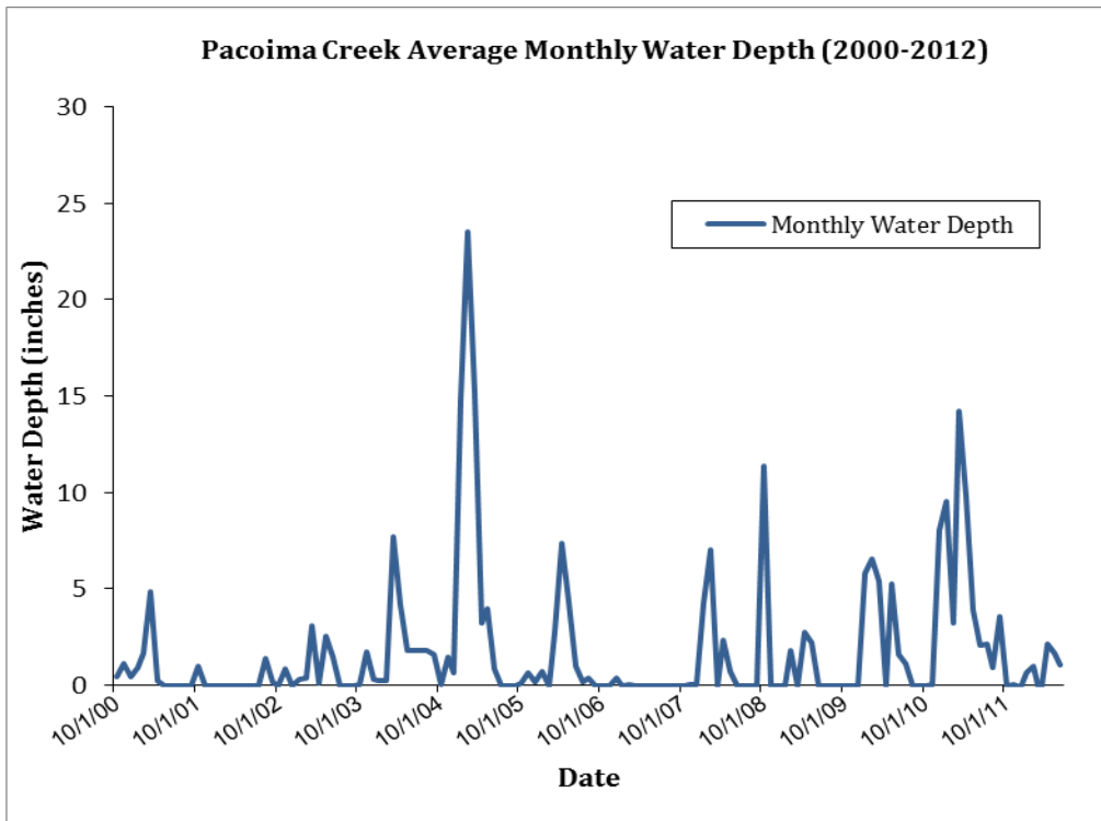
FIGURE 5-4.4b MONTHLY AVERAGE FLOW IN PACOIMA WASH FROM 2000 TO 2012
