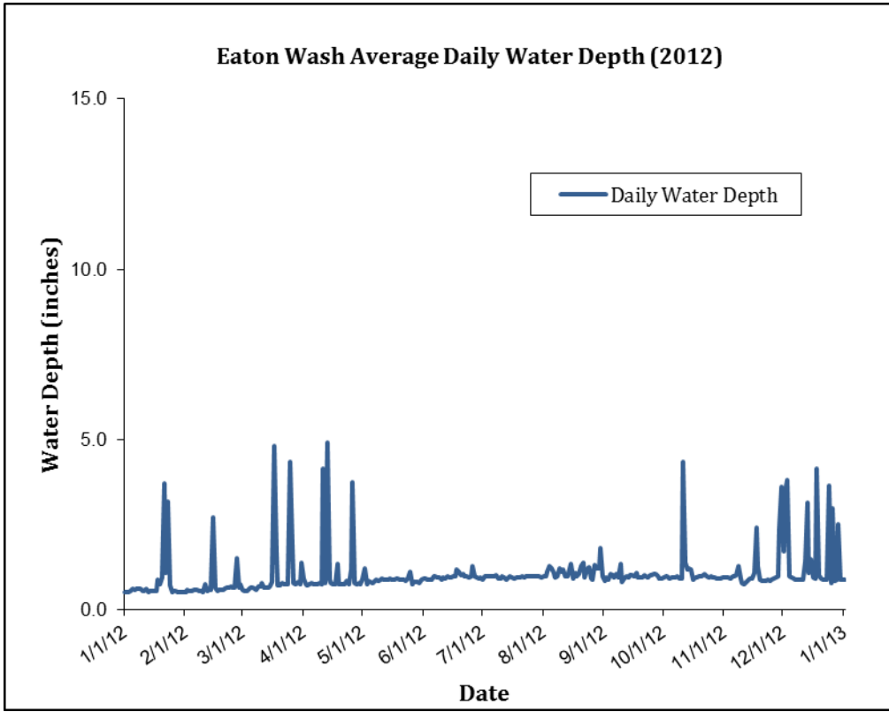
FIGURE 5-3.4a DAILY AVERAGE FLOW IN EATON WASH FOR THE YEAR 2012
